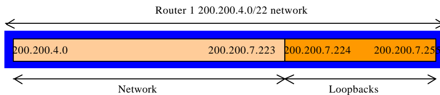
Figure 2 – Loopback Addressing Scheme: Picking the last /27 in the allocated block of /22
