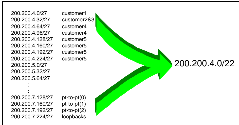
Figure 3 – Extract from ISP addressing plan
