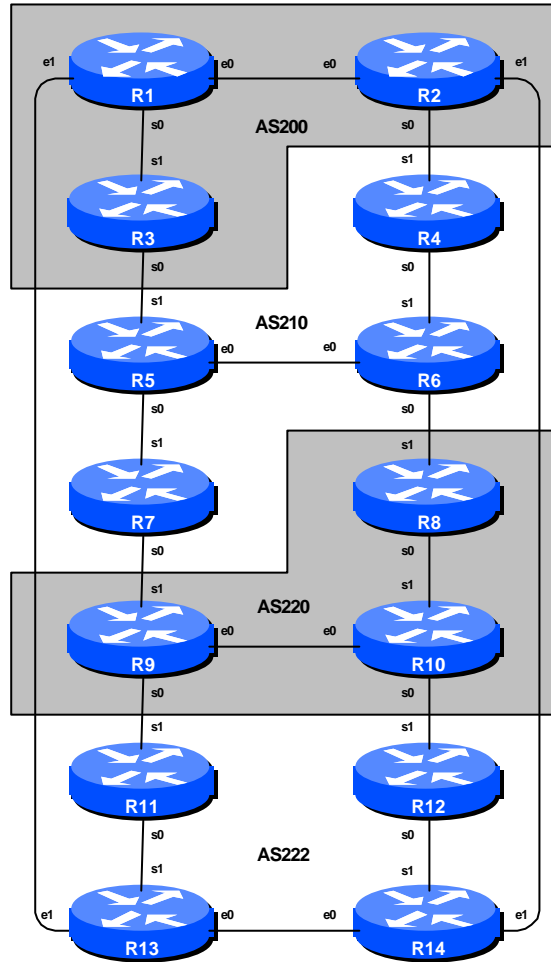
Figure 1 – BGP AS Numbers
