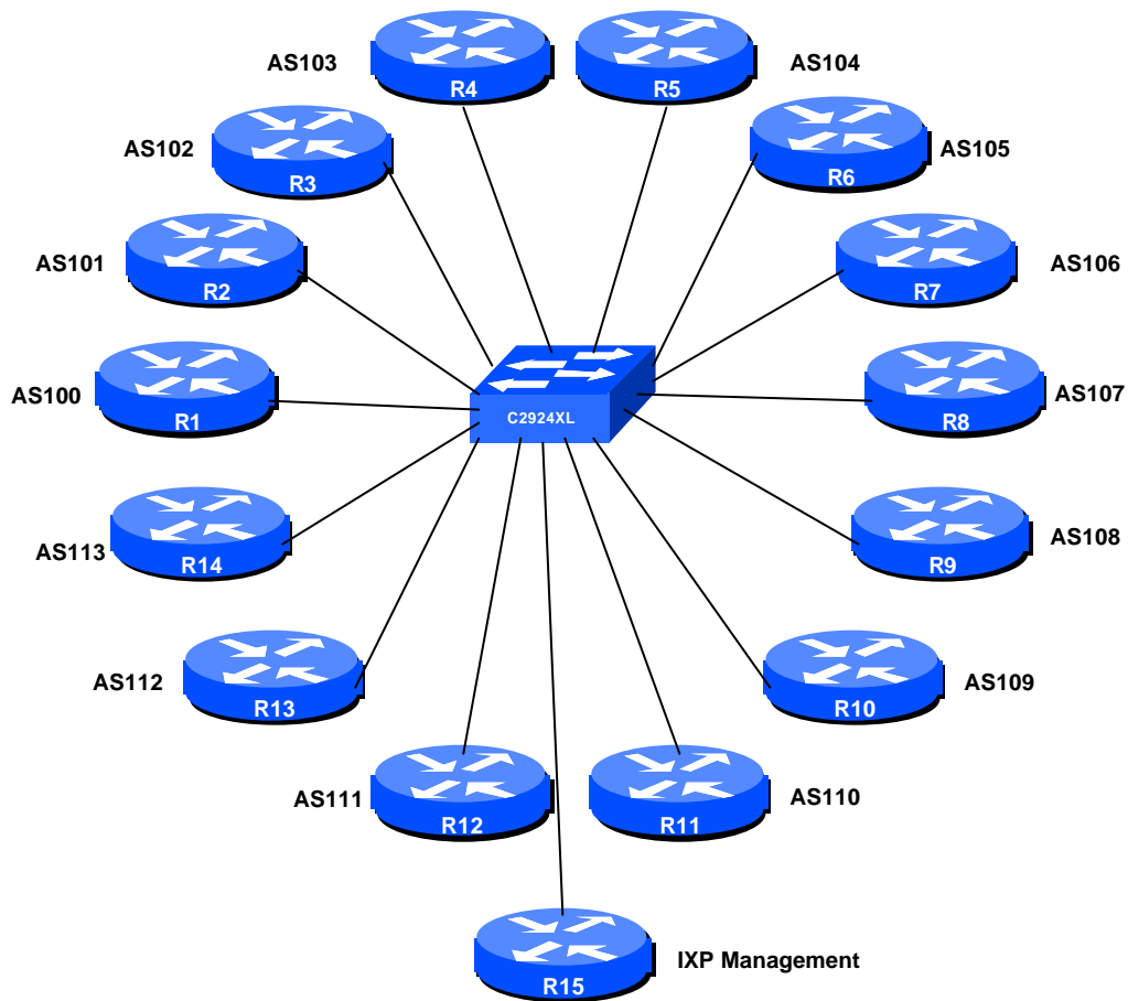
Figure 1 – IXP Configuration
